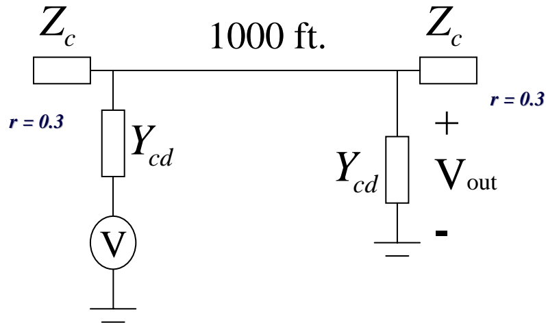
Point-to-point line with mismatch: Reflection coefficient = r
